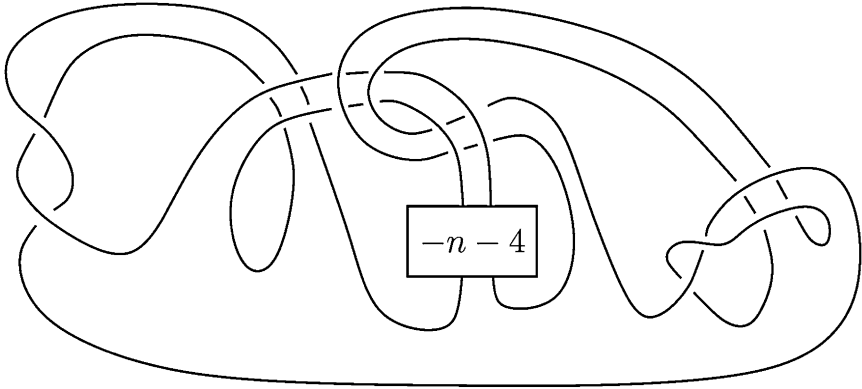
Figure 1 K_n
