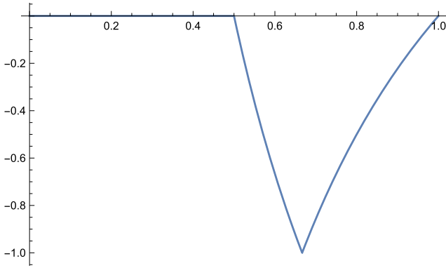
Figure 2 \Upsilon_{T(3,7)-T(4,5)}(t)/t
