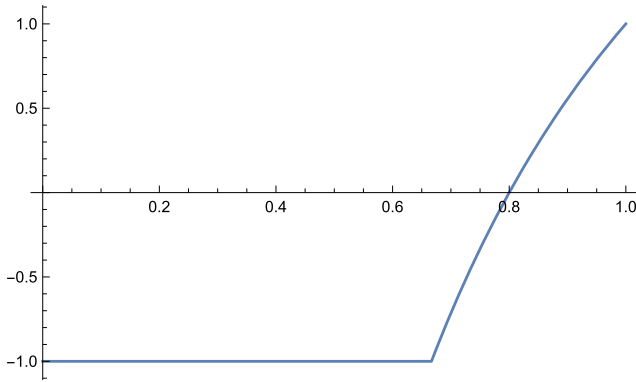
Figure 3 \Upsilon_{T(3,7)\#-T(2,11)}(t)/t
