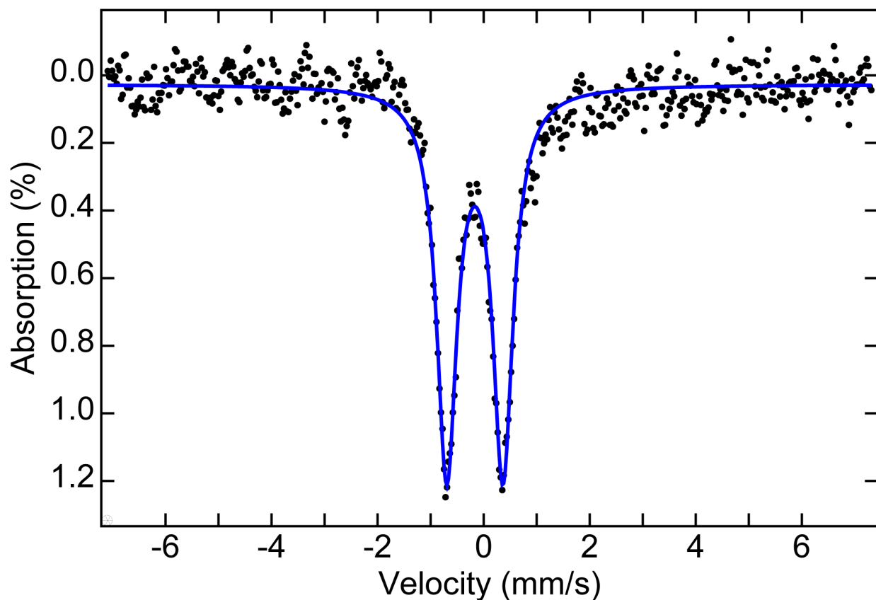
Figure 6. 57 Fe Mössbauer spectrum of 3 at 80 K. The blue trace is a simulation using \delta = -0.17 mm s -1 and \Delta E_Q = 1.06 mm s -1 .
