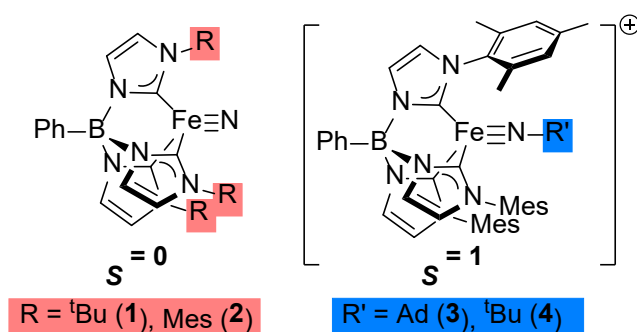
Figure 2. Iron(IV) nitrido (left) and imido (right) complexes supported by tris(carbene)borate ligands. In the nitrido complex, both R = \textit{tert} -butyl ( {}^t\text{Bu} , 1 ) and mesityl (Mes, 2 ) were investigated; for the imido complex, only R = \text{Mes} was studied, but with R' = \text{adamantyl} (Ad, 3 ) and \textit{tert} -butyl ( {}^t\text{Bu} , 4 ).
